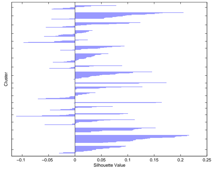
Fig. 3. Silhouette plot of the KNN cluster result. Each line represents an image. Lines on the right side of 0 measure how distant that image is from neighboring image sets. Lines on the left of 0 indicate that image is probably assigned to the wrong set. The vertical axis indicates different clusters (image sets).
