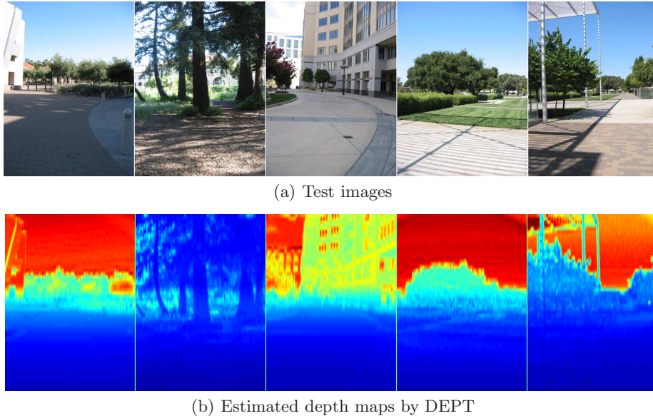
Fig. 1. Selected images and corresponding depth maps estimated by DEPT. The darker the red is, the further (from the imaging device) the objects are. The darker the blue is, the closer the objects are.
